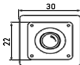
1. 3PIN WAFER TYPE (W/O AUDIO)
